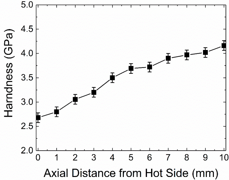
Figure 10: Vickers Micro Hardness axial traverse down the fully dense FGM ZnO.
