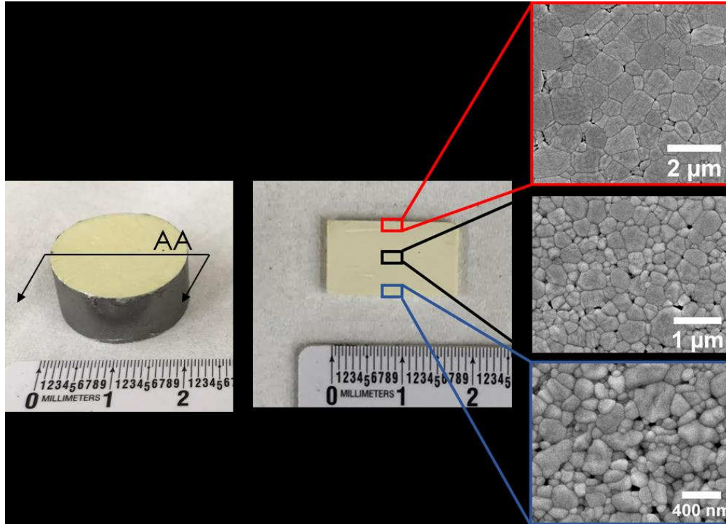
Figure 6: Macroscopic cross section and microscopic images of fully dense FGM ZnO.
